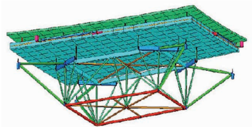
Fig. 7.18. The panel unit of the LMT. The red-green subframe is connected to the BUS by 4 actuators (shown in blue on the green spars). The cyan rectangle with 4 blue beams is the isostatic structure providing axial support of the panel baseplate (light blue). The green top layer is the reflecting surface.
