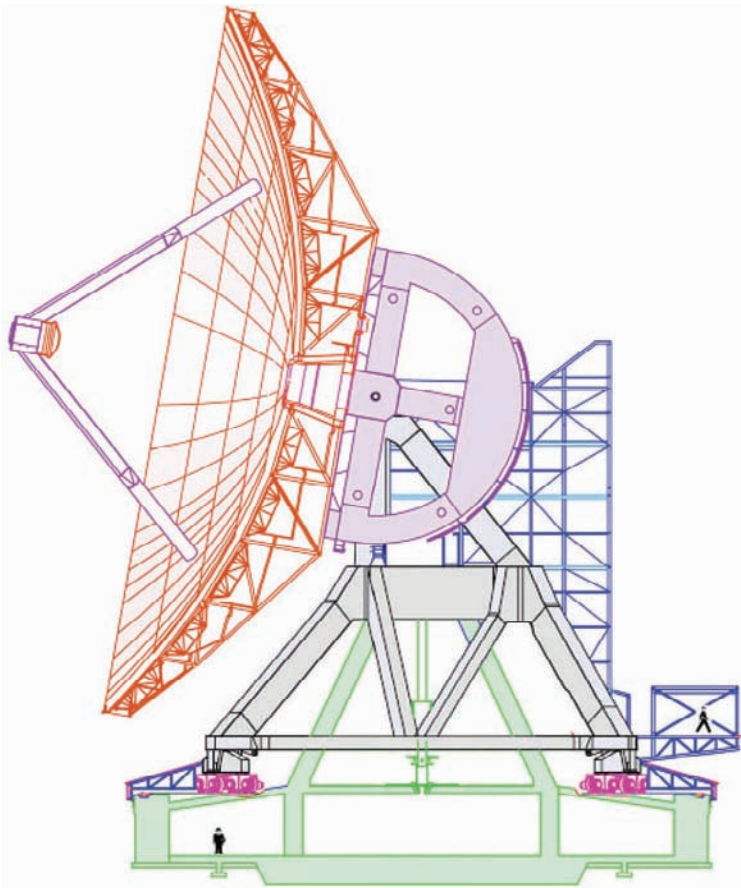
Fig. 7.16. Cross-section through the LMT. The green concrete foundation carries the antenna on 4 bogies and a bearing atop the central concrete pier. The alidade (gray) and elevation section (purple) are made of steel, as are the BUS (brown) and quadripod. Note the man in the basement for scale. (Drawing LMT Project)
