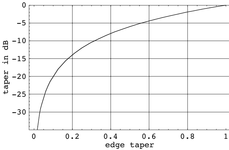
Fig. 4.2. The edge taper in dB against the value of \tau .
