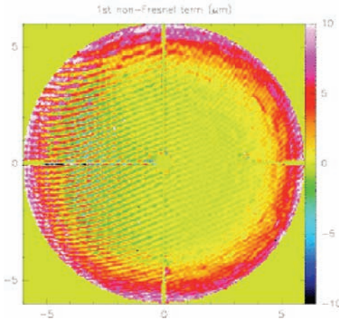
Fig. 6.6. Illustration of the higher order (non-Fresnel, Eq. (6.13)) phase error over the aperture. Over most of the aperture the error is about 2 \mu\text{m} ; it raises to more than 5 \mu\text{m} towards the edge.
