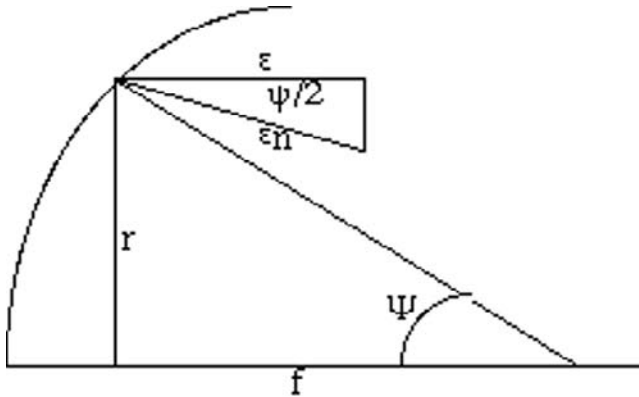
Fig. 4.20. Illustration of the relation between normal surface error \epsilon_n and the axial component \epsilon . The induced phase error is proportional to the latter.
