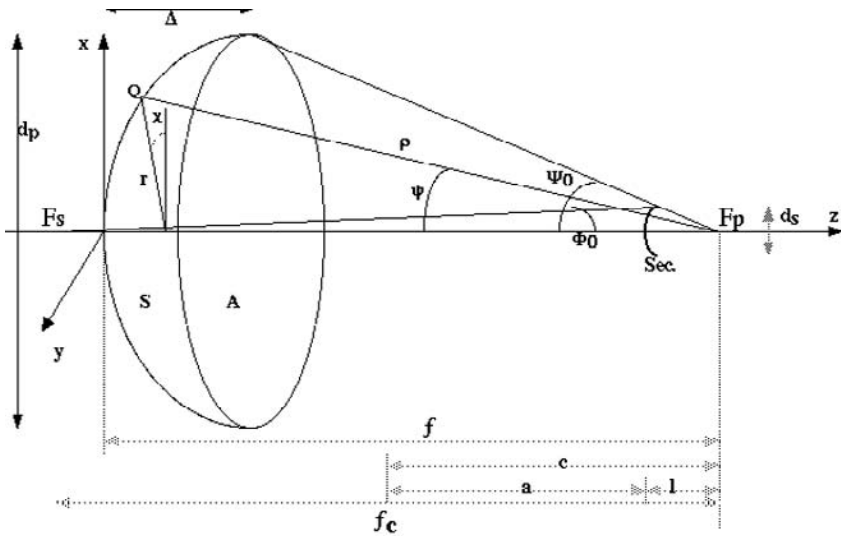
Fig. 2.2. Geometry of the Cassegrain reflector antenna
