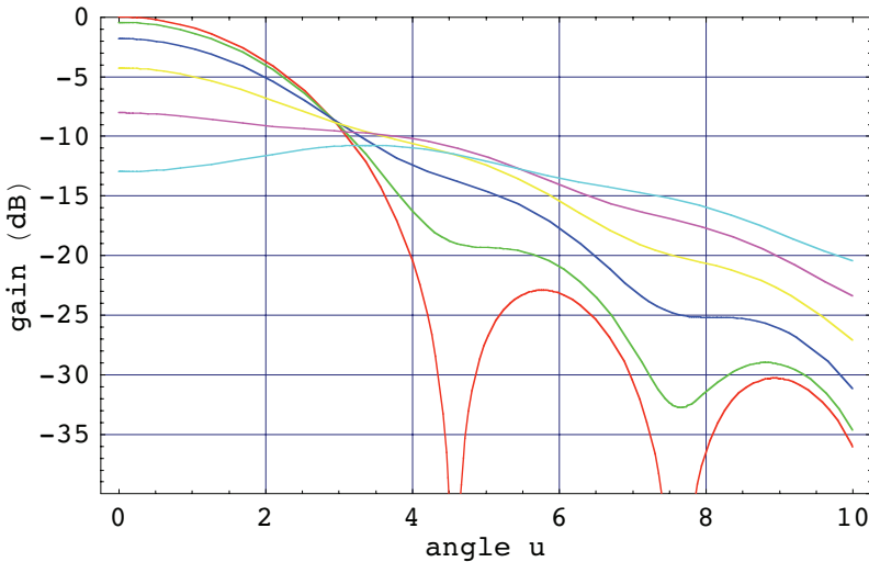
Fig. 4.12. A set of beam patterns for different values of axial defocus and a quadratic illumination function with edge taper of -12 dB. The defocus is in steps of 1 mm from 0 to 5 and the wavelength is 3 mm. The upper curve (red) applies to the focused case.
