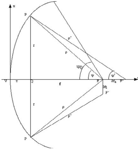
Fig. 6.5. The geometry of axial (upper half) and lateral (lower half) displacement of the feed from the focus of a parabola.
