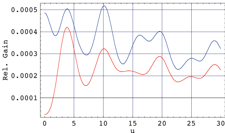
Fig. 6.24. Nearfield radiation function at a distance of 1/128 (blue) and 1/160 (red) times the farfield distance. Note the zero axial value of the red curve.
