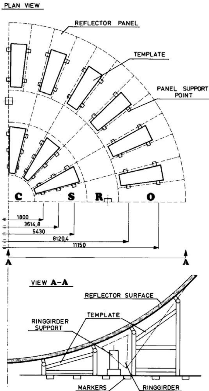
Fig. 7.6. The template for the assembly of the reflector in the assembly hall, consisting of two concentric rings of support beams with accurately located support points for the panels. Before the reflector was assembled the ring girder was placed inside the template, supported on 4 pillars, mimicking the 4 corners of the declination cradle.
