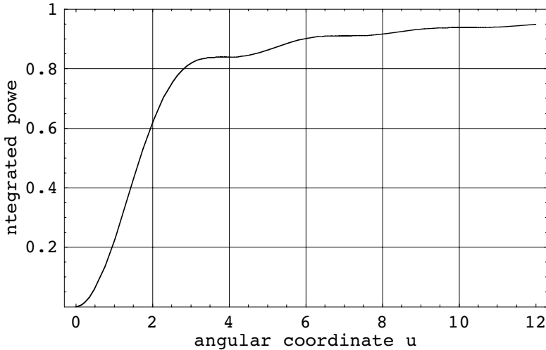
Fig. 3.5. The integrated power in the diffraction pattern as function of the angular coordinate. The plateaux near the minima in the pattern at u = 3.8 and 7.0 are clearly visible. The main beam contains 84 percent of the power.
