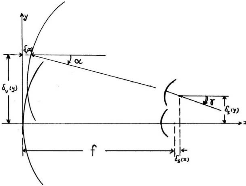
Fig. 5.11. Geometry of the different bulk displacements and rotations of the reflectors of a Cassegrain antenna system.
