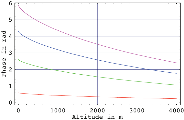
Fig. 6.21. Phase fluctuation as function of the altitude between two points 100-step 500-1600 m apart, from bottom to top.
