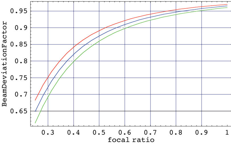
Fig. 4.17a. The BDF for fully tapered (red) and uniform (green) illumination as function of the focal ratio of the reflector. The middle curve (blue) is for a value of \tau = 0.25 (-12 dB) taper.
