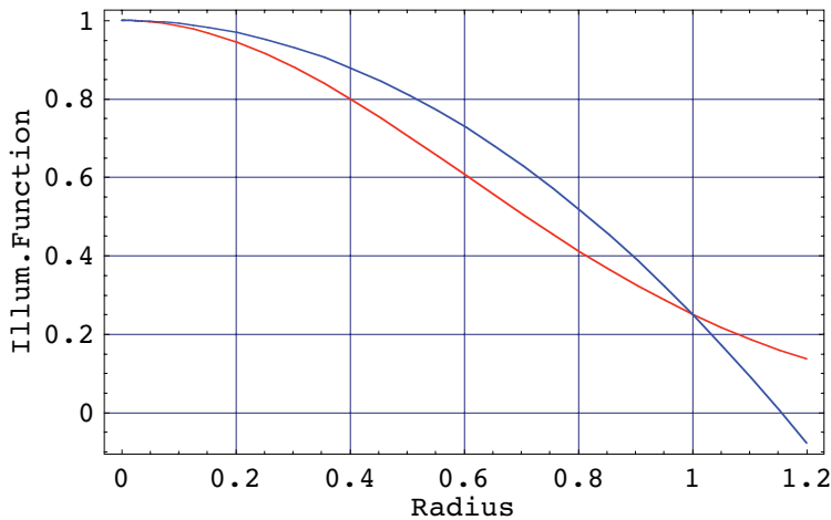
Fig. 4.3 The illumination function for the gaussian (red) and quadratic (blue) distribution and an edge taper of -12 dB. The quadratic illumination is somewhat more effective.
