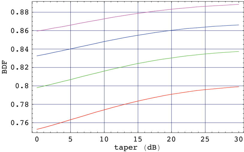
Fig. 4.17b. The beam deviation factor (BDF) as function of taper for f/D=0.35 -red, 0.4-green, 0.45-blue, 0.5-magenta.
