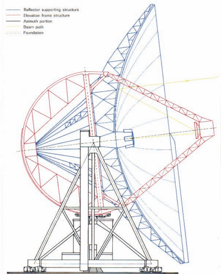
Fig. 7.8. Cross-section through the Effelsberg 100-m telescope. The reflector support structure (blue) is highly symmetrical and is connected to the elevation octahedron (red) at two points only. The octahedron is supported at two elevation bearings by the alidade (black), which runs on a 64 m diameter railtrack. (Drawing Krupp)
