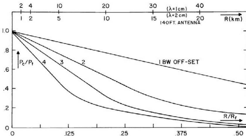
Fig. 6.25. The normalised beam overlap as function of the distance from the aperture in terms of the Rayleigh distance R_r , with the offset of the second beam in HPBW as parameter. The top scale indicates real distance for a 43-m diameter antenna and wavelengths of 1 and 2 cm.
