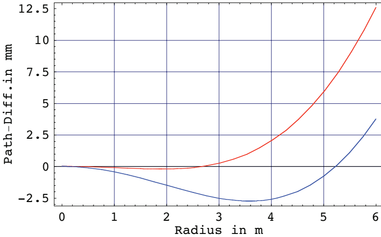
Fig. 6.2. The sum of the terms \delta_p and \delta_e for values \delta f = 80 mm (red) and 96 mm (blue). The aperture phase distribution must be corrected according to these residuals.
