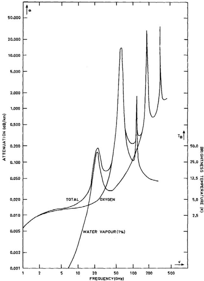
Fig. 6.19. Attenuation in the horizontal surface layer of the troposphere for oxygen, water vapour (assumed relative vapour density of 1%) and the total atmosphere. Right hand scale is atmospheric brightness temperature looking straight up for a standard atmospheric model.
